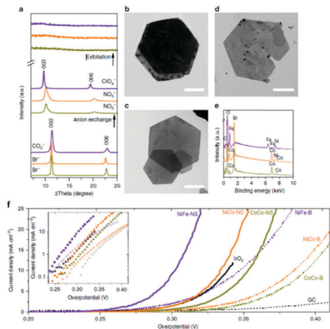
Fig. 13 (a) XRD spectra. (b–d) TEM images of (b) CoCo LDH–Br. Scale bar, 1 μm. (c) NiCo LDH–Br. Scale bar, 1 μm. (d) NiFe LDH–CO 3 2– . Scale bar, 150 nm. (e) Energy-dispersive X-ray spectra. CoCo LDH: yellow-green lines; NiCo LDH: orange lines; NiFe LDH: purple lines. (f) Polarization curves. Inset shows the Tafel plots. Scan rate was 5 mV s –1 . The loading was about 0.07 mg cm –2 for LDH materials and 0.21 mg cm –2 for IrO 2 nanoparticles. (Reproduced with permission (ref. 67) Copyright Nature Publishing Group (2014).)
