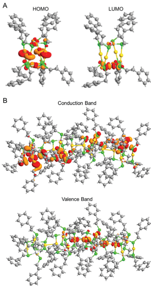
Fig. 7 (A) HOMO (left) and LUMO (right) states of an individual \mathbf{e} and (B) \Gamma -point Bloch wave functions for the conduction band minimum and valence band maximum of the 1D-CS of \mathbf{e} .
