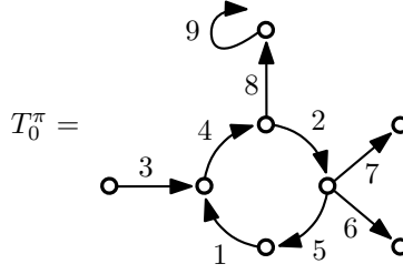
FIGURE 2. The quotient T_0^\pi for K = 9 and \pi = \{ \{1, 3, 13\}, \{2, 14, 15, 16\}, \{4, 11, 17\}, \{5, 10\}, \{6\}, \{7\}, \{8, 9, 18\}, \{12\} \} . For instance, the first block \{1, 3, 13\} means that the following vertices are equal: the targets of the 1st and 3rd edges and the source of the 4th edge (since 4 = 13 - 9 = 13 - K ).
