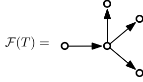
FIGURE 3. The graph of two-edge connected components of the graph T_0^\pi of Figure 2.
