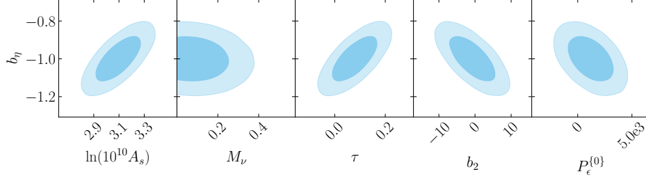
Figure 8: Contours showing the relationship between b_\eta and a subset of the other parameters in our calculations, for the central redshift bin of the combined galaxy clustering Euclid forecast (without CMB lensing). Apart from M_\nu , these parameters include those with the most significant (anti-)correlation with b_\eta . Despite some degree of correlation between b_\eta , A_s and \tau , the effect of varying b_\eta on the constraint on M_\nu is quite mild.
