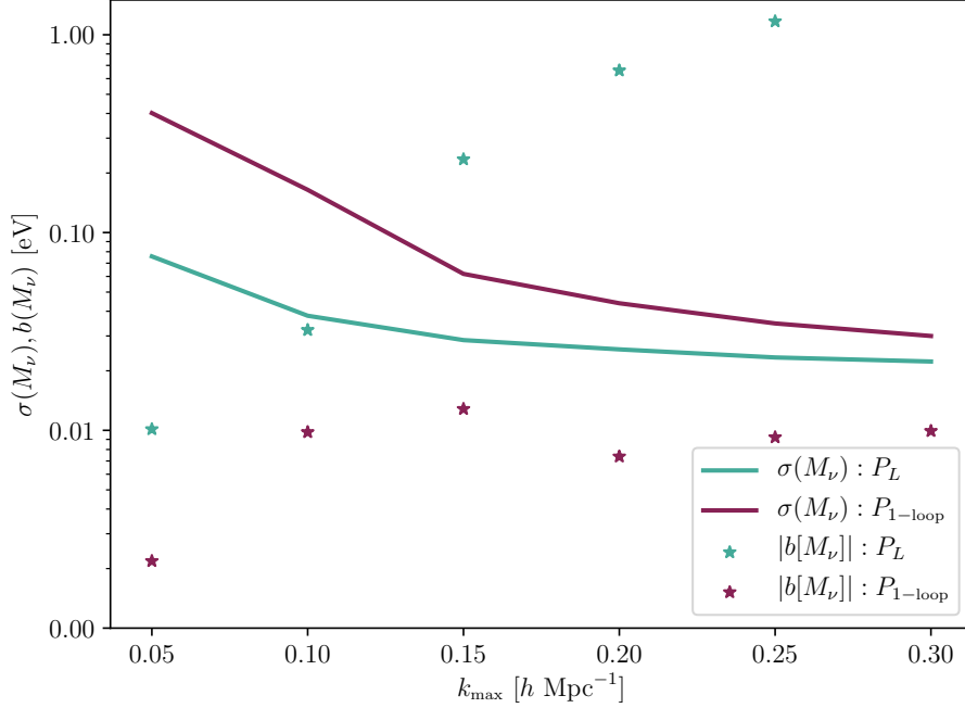
Figure 9: The forecasted 1\sigma constraints on M_\nu obtained using the linear (teal line) and 1-loop (purple line) galaxy power spectra for various k_{\text{max}} . The corresponding parameter biases resulting from not going to the next highest order in both cases are shown as points. The biases on M_\nu in the linear case are actually negative. In the 1-loop case, the biases are relatively small and fluctuate between positive and negative depending on the cut-off scale. This explains why the bias does not monotonically increase with k_{\text{max}} . At k_{\text{max}} = 0.2 \text{ h Mpc}^{-1} , the value we use in our calculations, the 1-loop bias is approximately 20% of the constraint.
