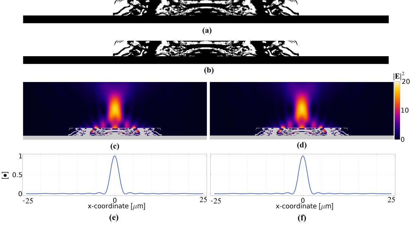
FIG. 4: (a) Design field, \xi(\mathbf{r}) , obtained by solving the optimization problem in eq. (16), black(white) corresponds to \xi = 1(\xi = 0) . (b) Thresholded design field, \xi(\mathbf{r}) > 0.5 . (c-d) The electric field intensity |\mathbf{E}|^2 (thermal) with the metalens overlaid (gray) for the (c) optimized design in (a) and (d) the thresholded design in (b) . (e-f) The max-normalized power flow through the focal plane for the (e) optimized design in (a) and (f) the thresholded design in (b) .
