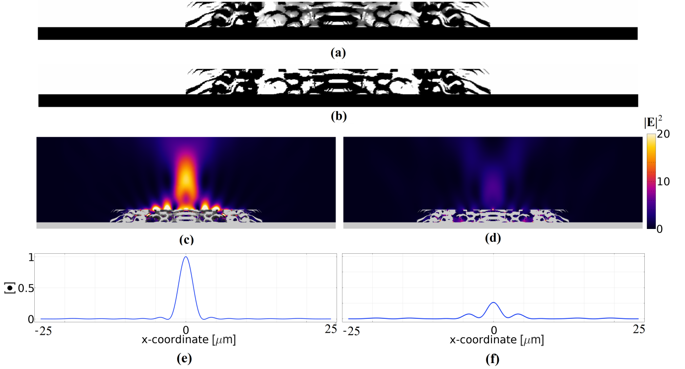
FIG. 3: (a) Design field, \xi(\mathbf{r}) , obtained by solving the optimization problem in eq. (14), black(white) corresponds to \xi = 1(\xi = 0) . (b) Thresholded design field, \xi(\mathbf{r}) > 0.5 . (c-d) The electric field intensity |\mathbf{E}|^2 (thermal) with the metalens overlaid (gray) for the (c) optimized design in (a) and (d) the thresholded design in (b) . (e-f) The max-normalized power flow, \langle \mathbf{P} \rangle , through the focal plane for the (e) optimized design in (a) and (f) the thresholded design in (b) .
