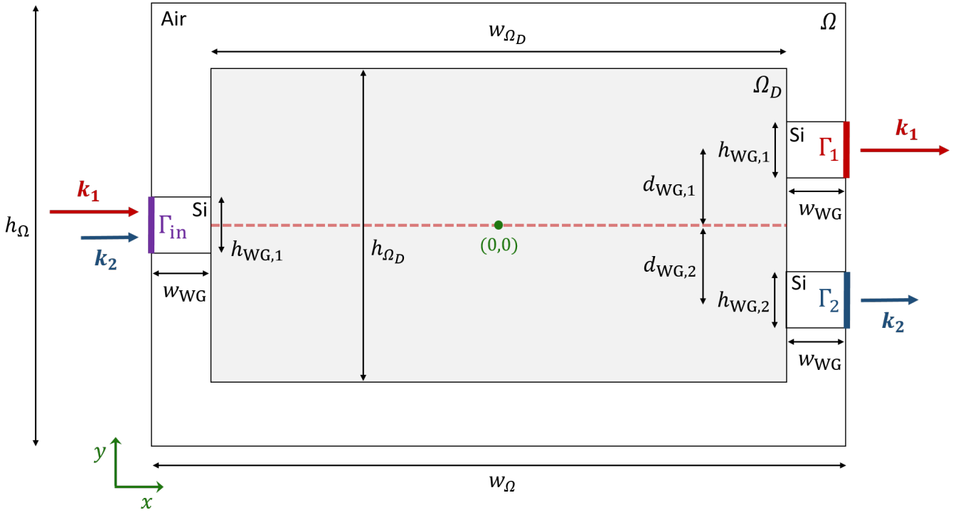
FIG. 7: The model domain \Omega considered in Sec. IX. Values for the lengths are found in Tab. IV.
