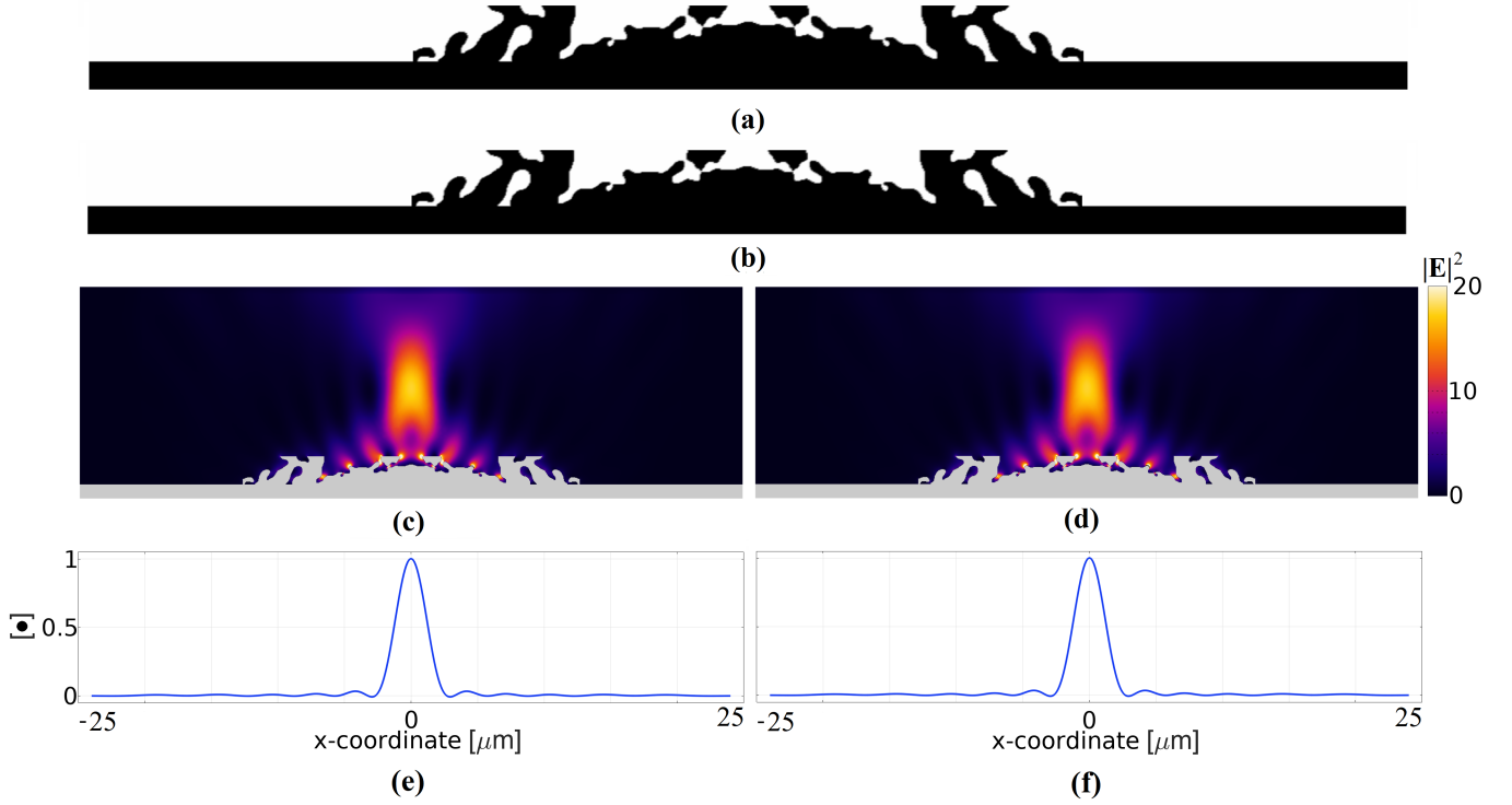
FIG. 5: (a) Design field, \xi(\mathbf{r}) , obtained by solving the optimization problem in eq. (19), black(white) corresponds to \xi = 1(\xi = 0) . (b) Thresholded design field, \xi(\mathbf{r}) > 0.5 . (c-d) The electric field intensity |\mathbf{E}|^2 (thermal) with the metalens overlaid (gray) for the (c) optimized design in (a) and (d) the thresholded design in (b). (e-f) The max-normalized power flow through the focal plane for the (e) optimized design in (a) and (f) the thresholded design in (b).
