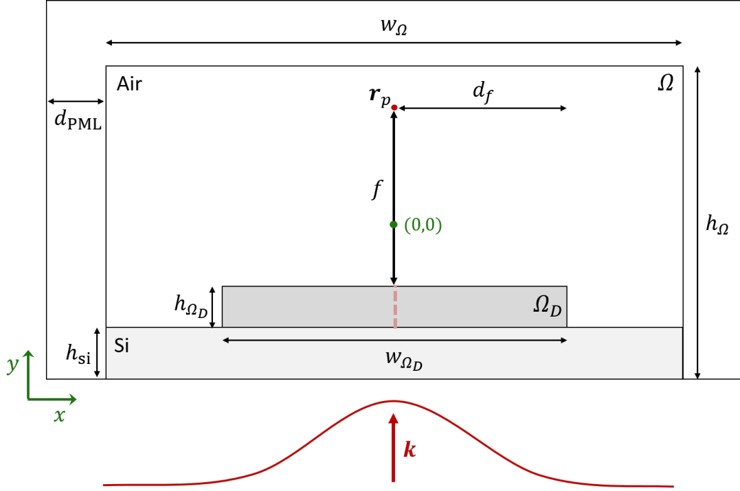
FIG. 2: The model domain, \Omega , used for the examples in sections VIII A-VIII D. Values for all lengths defined in the sketch are found in Tab. I.
