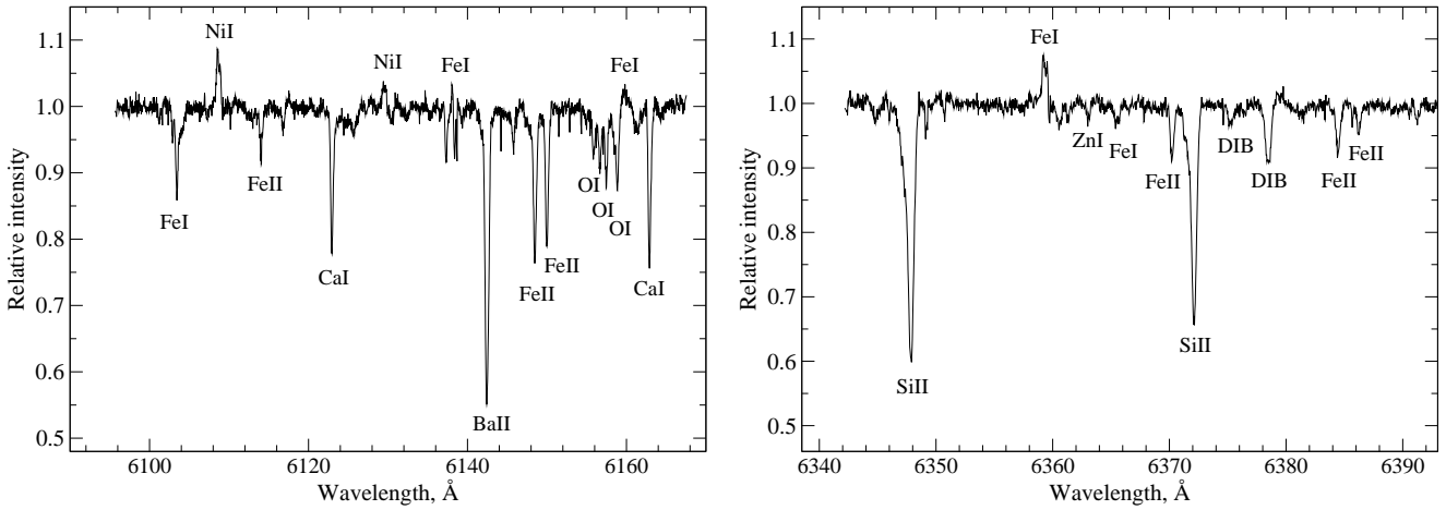
Figure 4. Fragments of the spectrum for V340 Ser containing peculiar features: FeI and NiI emissions as well as strong SiII(2) 6347 and 6371 Å absorptions with an extended blue wing and DIBs in the right fragment. The identification of the main features is indicated.
