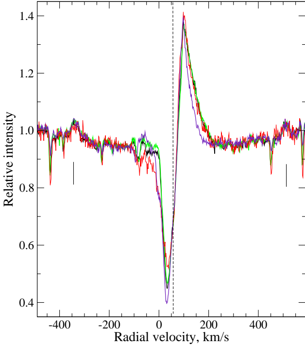
Figure 1. H\alpha profile in relative intensity – radial velocity coordinates in the spectra of V340 Ser taken at different dates: April 5, 2018 (black line), April 11, 2018 (green line), March 31, 2019 (red line), and April 2, 2020 (indigo line). The two solid vertical bars indicate the positions of the TiI 6554.23 Å and CaI 6572.80 Å emissions. The vertical line marks the systemic velocity \gamma = 56.8 \pm 0.5 km/s from de Smedt et al. (2016).
