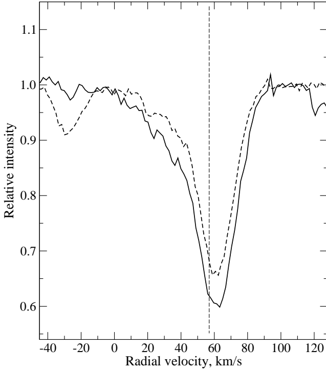
Figure 5. SiII(2) 6347 (solid line) and 6371 Å absorption profiles in the April 11, 2018 spectrum of V340 Ser. The vertical line marks the systemic velocity \gamma = 56.8 \pm 0.5 km/s (de Smedt et al., 2016).
