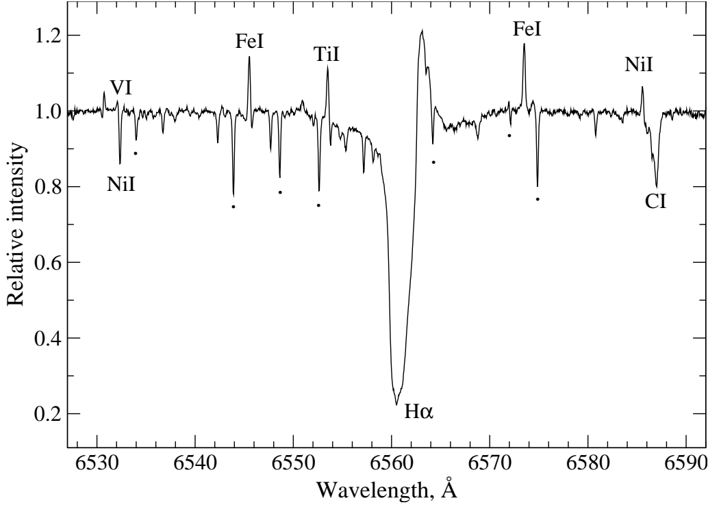
Figure 3. Fragment of the spectrum for 89 Her containing H \alpha and TiI, VI, FeI, and NiI emissions. The identification of the main absorptions is indicated. The dots mark the telluric features.
