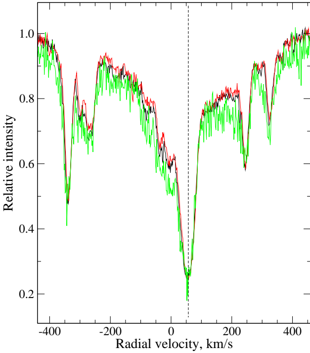
Figure 2. H\beta profile in the spectra of V340 Ser taken at different dates: April 5, 2018 (black line), April 11, 2018 (green line), and March 31, 2019 (red line). The vertical line marks the systemic velocity \gamma = 56.8 \pm 0.5 km/s from de Smedt et al. (2016).
