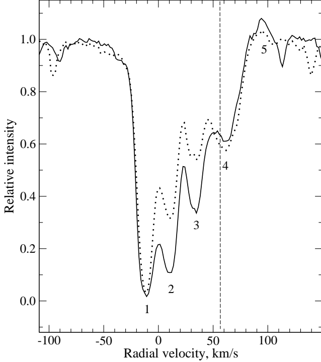
Figure 6. NaI 5889 and 5895 Å line profiles (dots) in the spectrum of V340 Ser. The positions of the profile absorption components forming in the interstellar medium (1), the circumstellar medium (2 and 3), and the stellar atmosphere (4) are marked. The vertical line marks the systemic velocity \gamma = 56.8 \pm 0.5 km/s (de Smedt et al., 2016).
