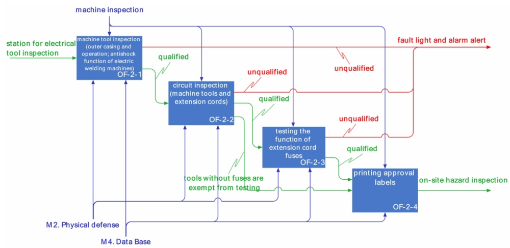
Fig. 5. Operation of electrical tool inspection station
