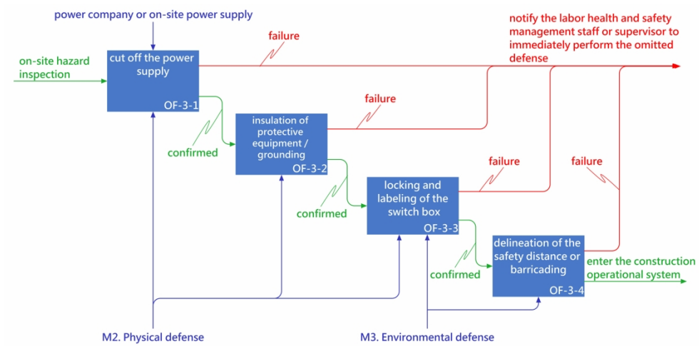
Fig. 6. Flowchart of on-site hazard inspection
