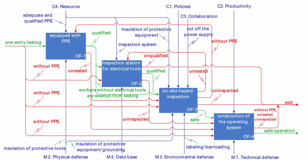
Fig. 4. Early intervention mechanism flowchart
