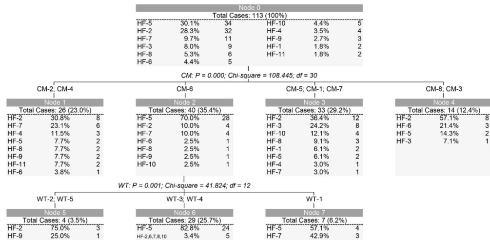
Fig. 2. Classification tree
