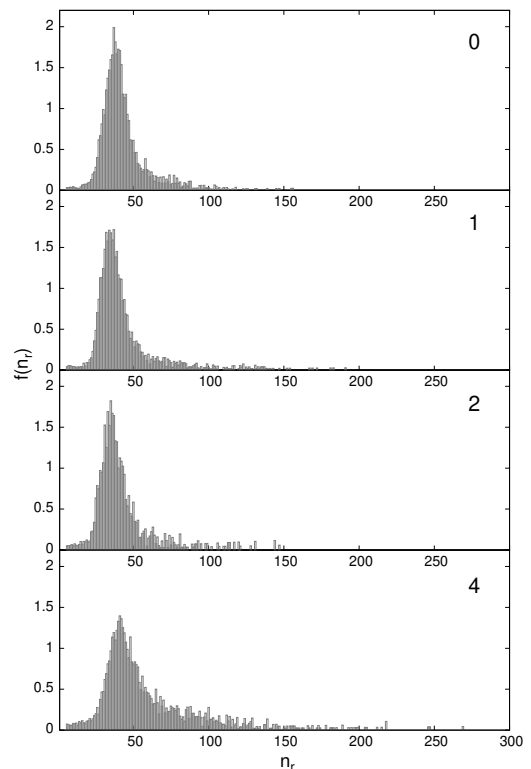
FIG. 5: Distribution of number of rods n_r in clusters containing more than five rods. From top to bottom: no obstacle, and obstacles of small, intermediate and large size. Labels indicate the diameter of the obstacle in cm.
