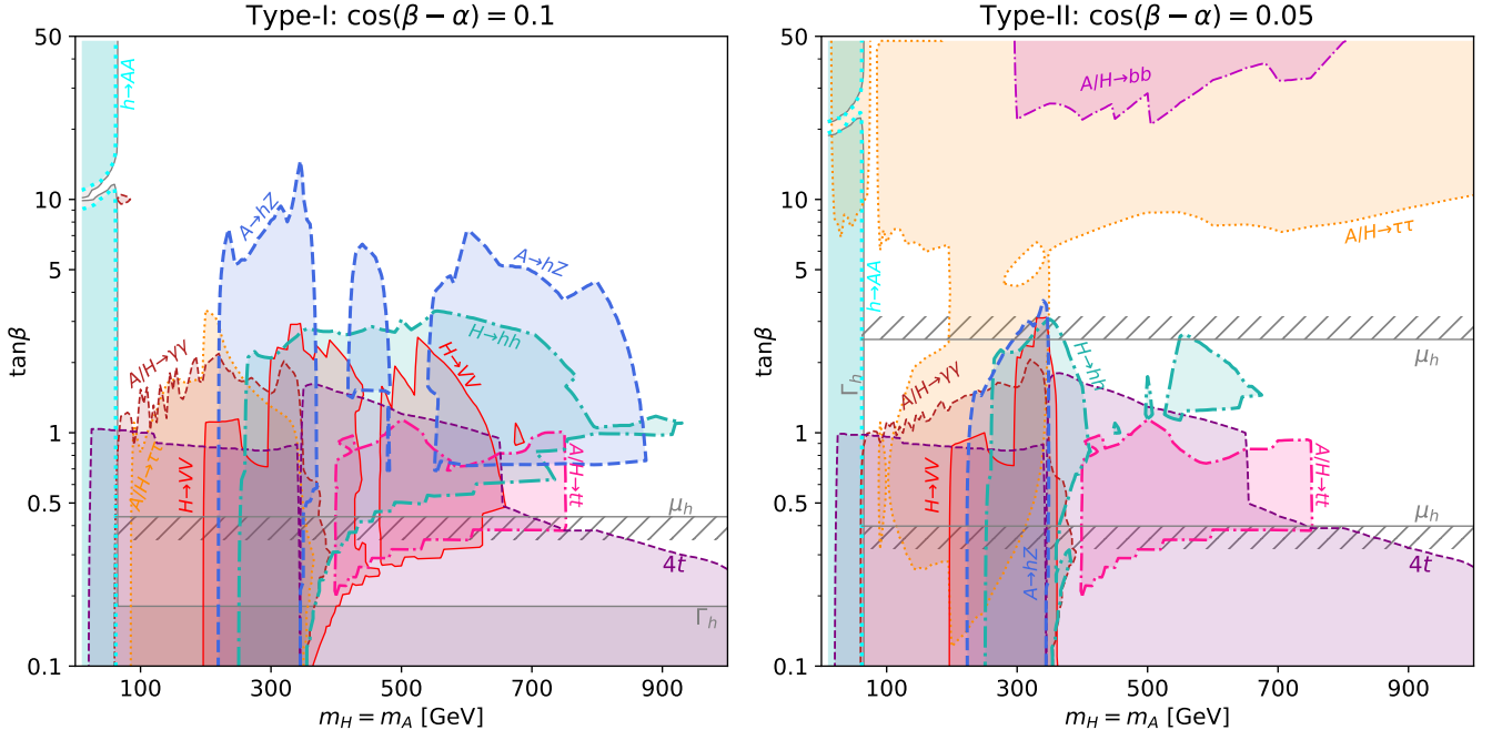
FIG. 1. Constraints for degenerate heavy Higgs mass spectrum m_A = m_H = m_{H^\pm} . We show the 95% C.L. exclusion region in the m_{A/H} vs. t_\beta plane on the Type-I 2HDM with c_{\beta-\alpha} = 0.1 (left) and Type-II 2HDM with c_{\beta-\alpha} = 0.05 (right) originating from i) the measurement of the Higgs width \Gamma_h (grey), ii) the conventional search results on H/A \rightarrow \tau\tau (dotted orange), H/A \rightarrow bb (dot-dashed pink), H \rightarrow VV (red), H/A \rightarrow \gamma\gamma (dashed brown), H/A \rightarrow tt (dot-dashed magenta) and 4t production (dashed purple), and iii) exotic decay channels A \rightarrow hZ (dashed dark blue), H \rightarrow hh (dot-dashed green) and h \rightarrow AA (dotted cyan). Region enclosed by the grey hatched line are excluded at 95% CL. by the current Higgs coupling measurements.
