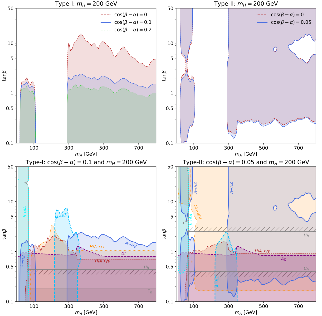
FIG. 4. Constraints on the Type-I (left panel) and the Type-II (right panel) 2HDM in m_A - t_\beta plane. Top: Parameter space excluded at 95% C.L. by the A/H \rightarrow HZ/AZ search for m_H = 200 GeV and c_{\beta-\alpha} = 0 (red), 0.1 (blue) and 0.2 (green) in the left panel and c_{\beta-\alpha} = 0 (red) and 0.05 (blue) in the right panel. Bottom: Constraints at 95% C.L. for m_H = 200 GeV and c_{\beta-\alpha} = 0.1 from LHC searches for A \rightarrow HZ (blue), A \rightarrow hZ (dashed dark blue), H \rightarrow AA (dashed cyan), H/A \rightarrow \tau\tau (dotted orange), H/A \rightarrow \gamma\gamma (dashed brown) and 4t production (dashed magenta) as well as the global fit of SM-like Higgs couplings strength \mu_h (grey hatched region) and the Higgs width measurement \Gamma_h \notin (0.08, 9.16) MeV (grey).
