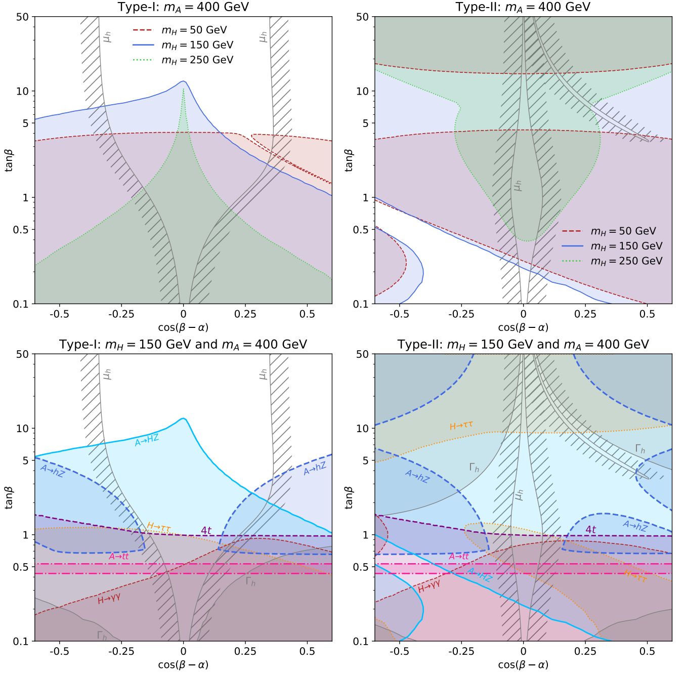
FIG. 3. Constraints on the Type-I (left panel) and the Type-II (right panel) 2HDM in t_\beta - c_{\beta-\alpha} plane. Top: Parameter space excluded at 95% C.L. by the A/H \rightarrow HZ/AZ search for m_A = 400 GeV and m_H = 50 GeV (red), 150 GeV (blue) and 250 GeV (green), and by the global fit of SM-like Higgs couplings strength \mu_h (grey). Bottom: Constraints at 95% C.L. for m_A = 400 GeV and m_H = 150 GeV from LHC searches for A \rightarrow HZ (blue), A \rightarrow hZ (dashed dark blue), H \rightarrow \tau\tau (dotted orange), H \rightarrow \gamma\gamma (dashed brown), A \rightarrow tt (dot-dashed magenta) and 4t production (dashed purple) as well as the global fit of SM-like Higgs couplings strength \mu_h (grey hatched region).
