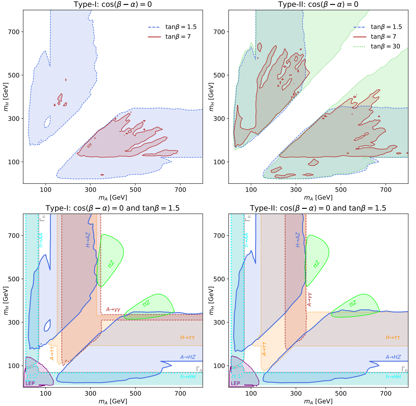
FIG. 2. Constraints on the Type-I (left panel) and the Type-II (right panel) 2HDM in m_A vs. m_H plane. Top: Parameter space excluded at 95% C.L. by the A/H \rightarrow HZ/AZ search in the alignment limit, c_{\beta-\alpha} = 0 , for t_\beta = 1.5 (blue), 7 (red) and 30 (green). Bottom: Constraints at 95% C.L. for c_{\beta-\alpha} = 0 and t_\beta = 1.5 from LHC searches for A/H \rightarrow HZ/AZ (blue), A/H \rightarrow \tau\tau (dotted orange), A/H \rightarrow \gamma\gamma (dashed brown), h \rightarrow AA/HH (dotted cyan) and ttZ production (green) as well as LEP searches (purple) and the Higgs width measurement \Gamma_h \in (0.08, 9.16) MeV (grey).
