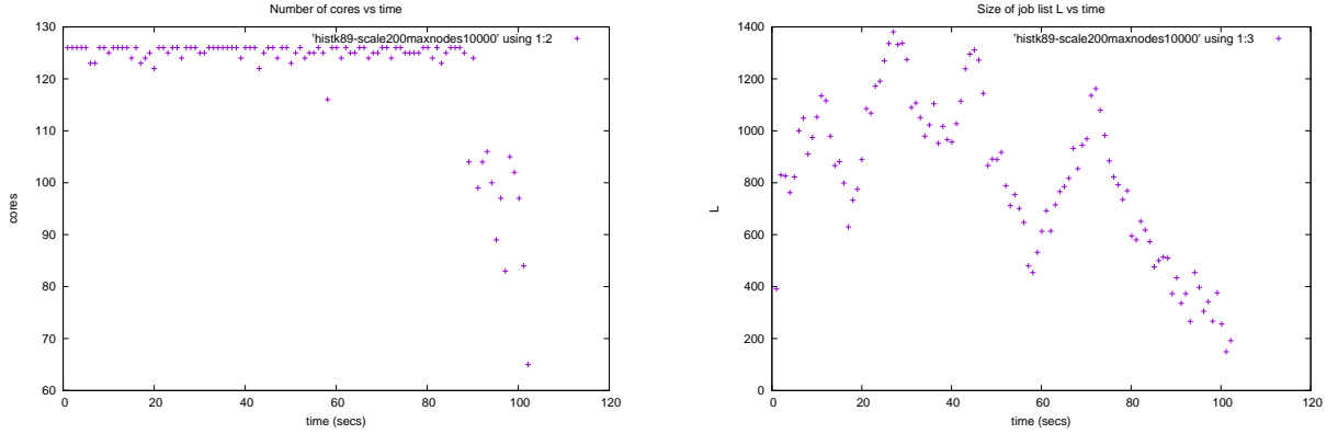
Figure 7: Histograms with -scale 200 -maxnodes 10000 on K_{8,9} : busy workers (l), joblist size (r)
