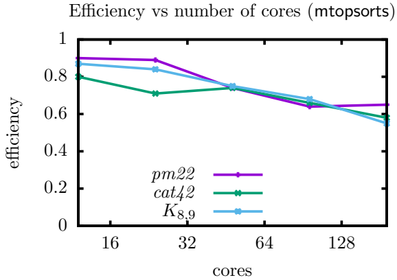
(a) Efficiency with mtopsorts
