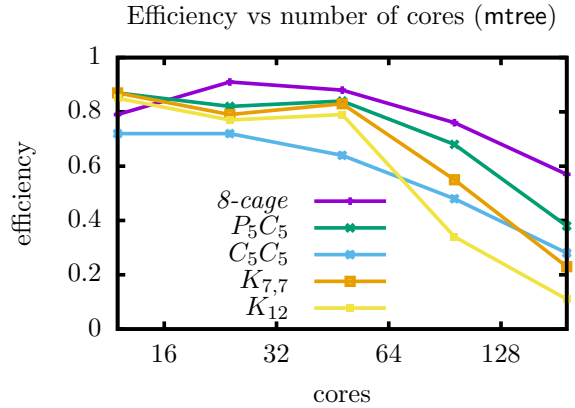
(b) Efficiency with mtree
