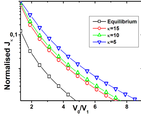
Figure 5: (color on line) Values of the transmited proton current density as a function of V_0/V_1 through a hill potential barrier at temperature T = 5000K , with V_1 = 0.5 \text{ eV} .
