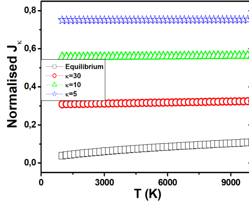
Figure 3: (color on line) Values of the transmited proton current density as a function of the temperature through a hill potential barrier of heighth V_1 = 200 \text{ eV} , V_0/V_1 = 1.3 .
