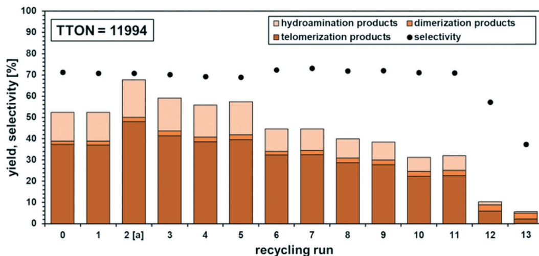
Fig. 6 Recycling experiments with Pd(acac) 2 /TPPTS system with an increased Pd:L ratio of 1:8. Conditions: 35 mmol (2.9 g, 3.6 mL) \beta -myrcene, 70 mmol (5.4 g, 5.1 mL) dimcarb, 0.035 mol% (0.8 mmol L -1 ) Pd(acac) 2 , n_{\text{Pd}}:n_{\text{TPPTS}} = 1:8 , T = 100^\circ\text{C} , 4 h, rpm = 500, and p_{\text{Ar}} = 0.01 MPa. After 1 h phase separation, 35 mmol \beta -myrcene and 13 mmol of dimcarb were added. Yield determined via GC-FID. [a]: t = 4.5 h.
