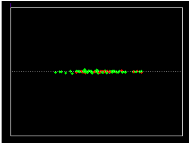
Figure 10: A simulation following the motion of 100 pulsars in a model gravitational potential of our Galaxy for 200 Myr. The view is edge-on, i.e. the horizontal axis represents the Galactic plane (30 kpc across) while the vertical axis represents \pm 10 kpc from the plane. This snapshot shows the initial configuration of young neutron stars.
