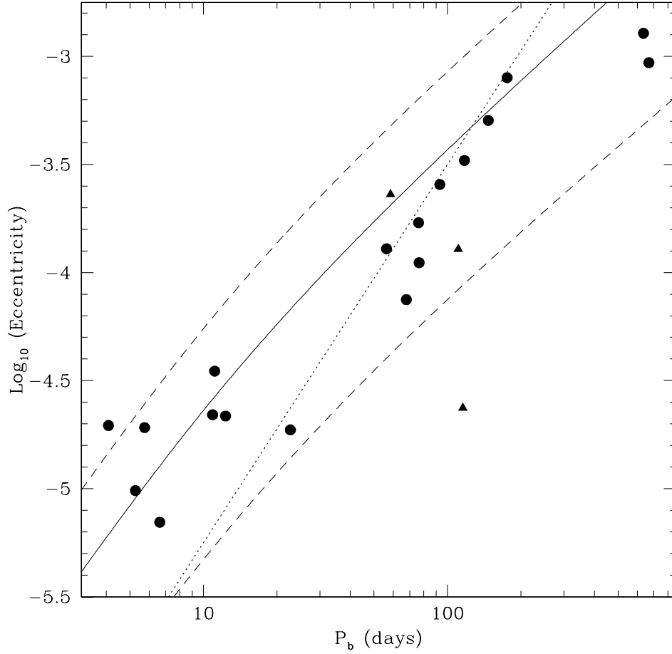
Figure 8: Eccentricity versus orbital period for a sample of 21 low-mass binary pulsars which are not in globular clusters, with the triangles denoting three recently discovered systems [347]. The solid line shows the median of the predicted relationship between orbital period and eccentricity [298]. Dashed lines show 95% the confidence limit about this relationship. The dotted line shows P_b \propto e^2 . Figure provided by Ingrid Stairs [347] using an adaptation of the orbital period-eccentricity relationship tabulated by Fernando Camilo.
