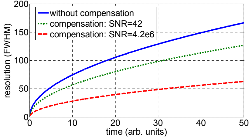
Fig. 18. Possible spatial resolution (FWHM) from a measured temperature profile after a certain time without compensation (solid line) and with compensation for a small signal- to-noise-ratio (SNR) from the data shown in Fig. 13 (dotted line) and a SNR of 4.2 \cdot 10^6 (dashed line).
