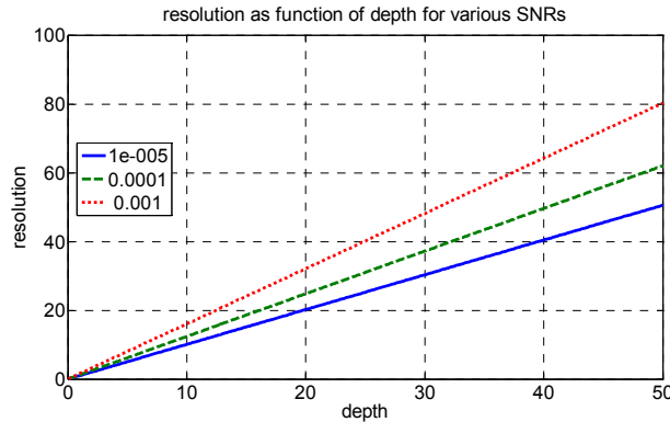
Fig. 23. Resolution as function of depth for various SNRs. The resolution is the smallest distance at which two different peaks can be resolved in the reconstructed temperature and is estimated by the distance of the two zero points near the peak at the depth (see also Fig. 22).
