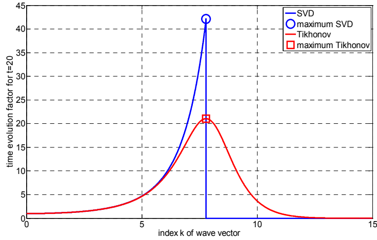
Fig. 15. Time evolution factor for the initial temperature profile shown in Fig. 13 for a time t=20 . At that time wave numbers increasing k=8 are determined by the fluctuations and have nearly no additional information about the initial temperature profile (Fig. 14).
