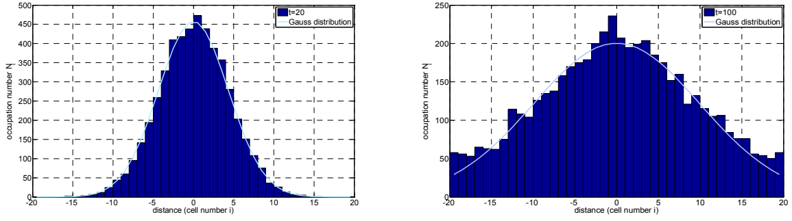
Fig. 3. Occupation number representation of the Wiener process for 5000 particles starting at x=0 at t=20 (left) and t=100 (right). For comparison the Gaussian distribution with a variance proportional to time is shown. For t=100 the reflecting boundaries at a distance of \pm 20 can be already recognized by occupation numbers significantly increasing the Gaussian distribution.
