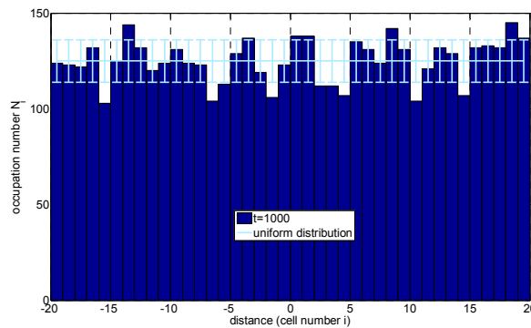
Fig. 4. Occupation number representation of the Wiener process for N=5000 particles starting at x=0 at t=1000 using 40 cells. At that time the influence of the reflecting boundaries at a distance of \pm 20 dominates. For comparison the uniform distribution with the mean value 125 (5000 particles divided by 40 cells) and the errorbar at \pm the standard deviation is shown. The standard deviation is the square root of the variance given in eq. (7) using p_i=1/40 for the uniform distribution.
