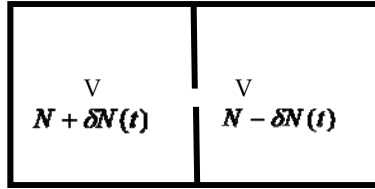
Fig. 7. Distribution of 2N particles between two boxes of volume V , which are connected by a small hole where particles can change between the two boxes at a constant time rate \gamma (effusion). At a certain time t , N + \delta N(t) particles are situated in the left box and N - \delta N(t) particles are in the right box.
