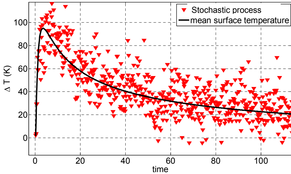
Fig. 21. Deviation from equilibrium temperature \Delta T = T - \bar{T} at the surface as a function of time, “measured” at a time step of \Delta t = 0.2 . The initial temperature distribution is Gaussian shaped with a maximum of 600 Kelvin (K) at a depth of 20 and the full width at 1/e of the maximum is 16 arb. units (compare Fig. 13). The minimum temperature is 300 K. The standard deviation at the surface is again constant in time.
