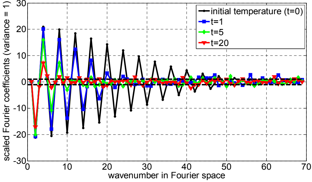
Fig. 14. Fourier coefficients as a function of time. Coefficients with a higher wavenumber show a rapid decay with time according to eq. (43). The Fourier coefficients are scaled to have a variance of one (independent of wavenumber).
