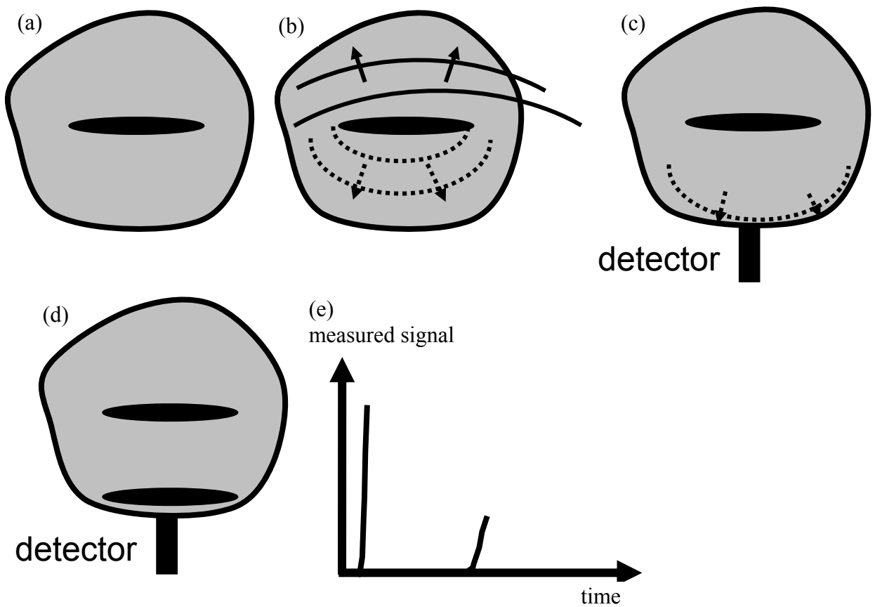
Fig. 1. Information loss in non-destructive imaging: the spatial resolution is essentially influenced by the propagation of certain waves, e.g. ultrasound or electromagnetic waves to the surface. Scattering, dissipation, or diffusion causes entropy production and a loss of information of the propagating waves. (a) Sample containing internal structure, which should be imaged. (b) Propagation of the waves to the sample surface: entropy production goes along with fluctuations (“fluctuation-dissipation theorem”, see text) and a loss of information. (c) Detection of wave at the sample surface. (d) The same structure is contained twice in the sample: just beneath the surface and at a higher depth. (e) Measured signal at the detector surface as a function of time for the sample shown in (d): due to diffusion or dissipation the signal from the deeper structure has not only smaller amplitude but it is also broadened compared to the signal from the structure just beneath the surface.
