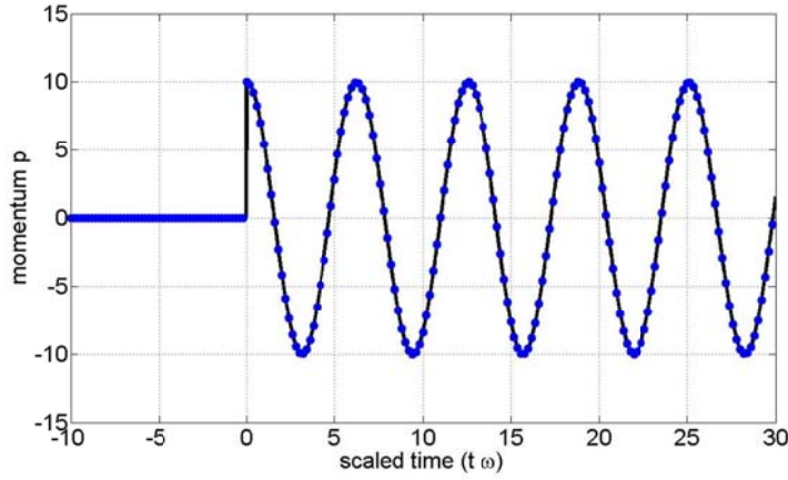
Fig. 8. Points on a sample path of the kicked harmonic oscillator without damping. The momentum used to kick the oscillator can be reconstructed without loss of information at any time t after the kick if \omega is known.
