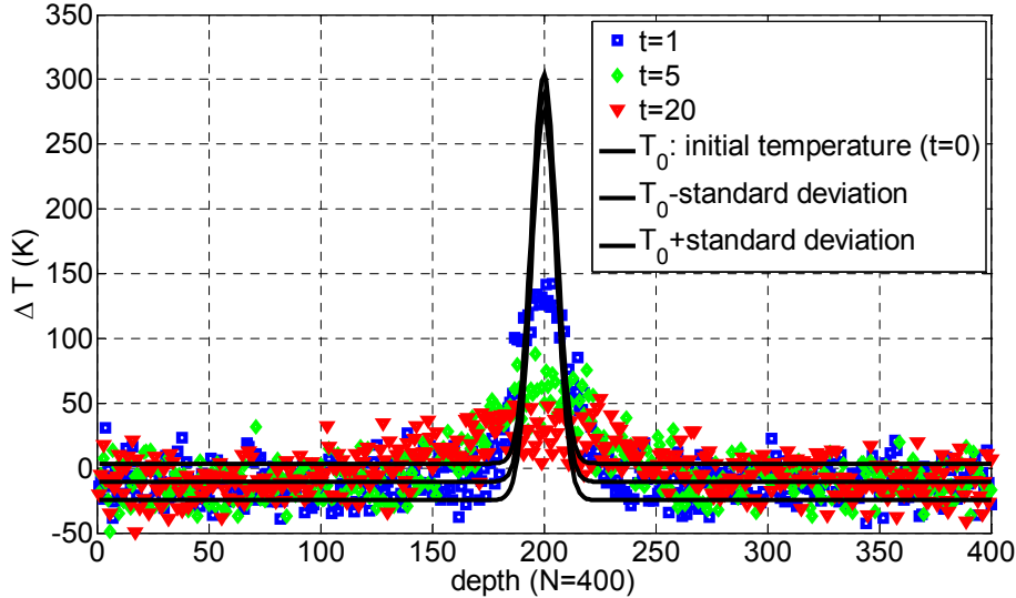
Fig. 13. Deviation from equilibrium temperature \Delta T = T - \bar{T} in real space as a function of time. The initial temperature distribution is Gaussian shaped with a maximum of 600 Kelvin (K) at a depth of 200 and the full width at 1/e of the maximum is 16 arb. units. The minimum temperature is 300 K. The standard deviation in real space (see text) is constant in depth and time.
