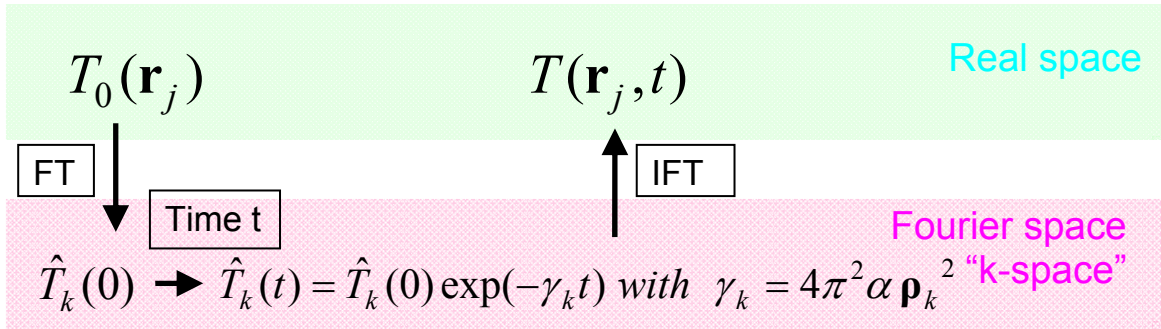
Fig. 12. The initial temperature distribution T_0(\mathbf{r}) just after the laser pulse is Fourier transformed (FT). The time evolution of the Fourier series coefficients can be described similar to the mean value of an Ornstein-Uhlenbeck process (eq. (15)). The temperature distribution T(\mathbf{r}, t) after a time t is then calculated by an inverse Fourier transform (IFT).
