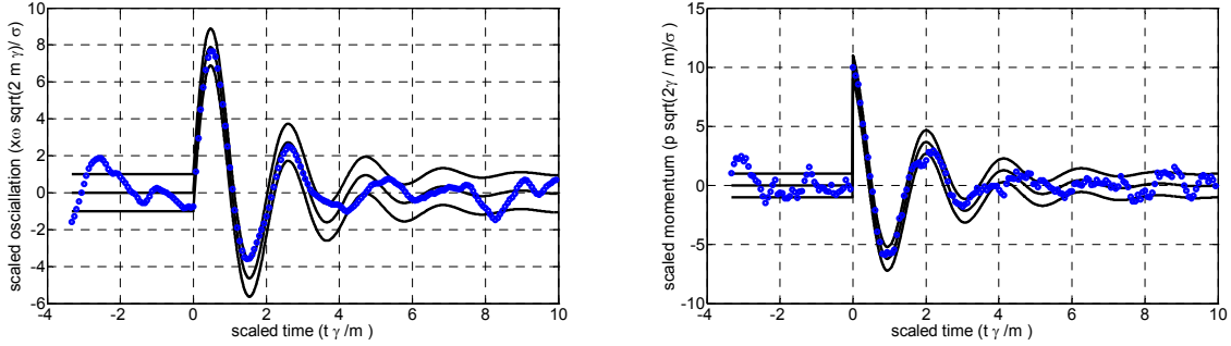
Fig. 9. Points on a sample path of the normalized kicked damped harmonic oscillator (eq. (24) and (25)). The solid lines represent the mean, and mean \pm standard deviation of the scaled oscillation (left) and momentum (right). At the time t=0 a value of p_0=10 has been added to the scaled momentum. After some time the information about the value of p_0 gets more and more lost due to the fluctuations.
