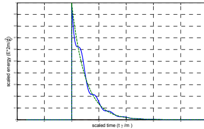
Fig. 10. Total energy of the damped harmonic oscillator (solid line) shows in the average an exponential decay with the time constant \gamma / m (dashed line).
