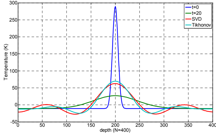
Fig. 16. Reconstruction using the time evolution factors from Fig. 15 for SVD and Tikhonov reconstruction.
