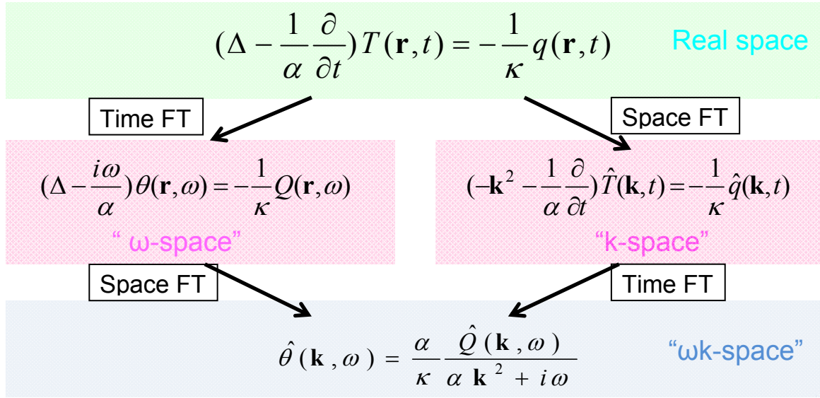
Fig. 11. The diffusion equation (34) can be solved by Fourier transform (FT) in time (eq. (35)) and a subsequent FT in space (eq. (37)). The same result in “ωk-space” is gained if the space FT is performed first, and then the time FT.
