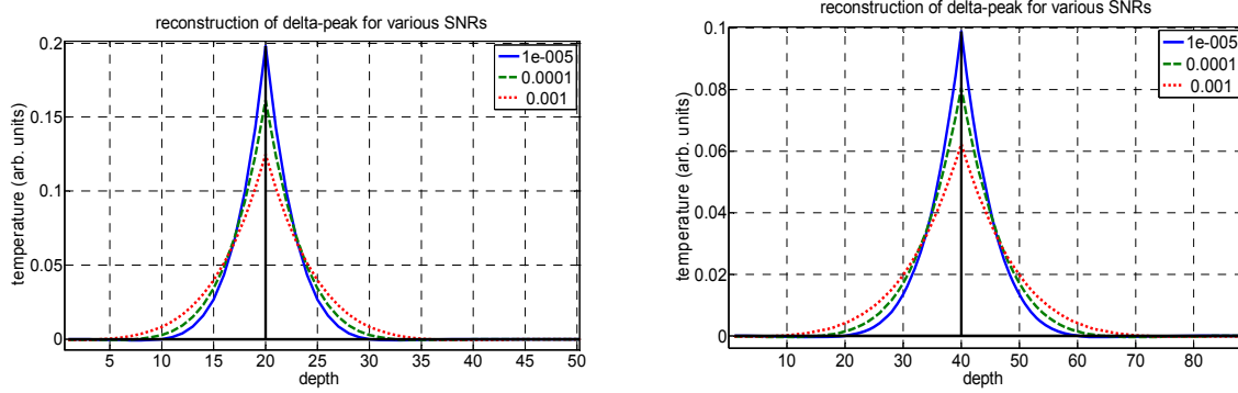
Fig. 22. Reconstruction of the temperature profile from a delta-source at a depth of 20 (left) and 40 (right) for three different noise levels.
