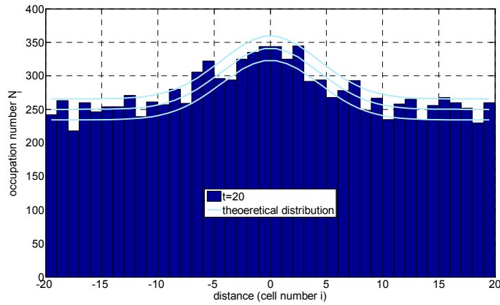
Fig. 5. Occupation number representation of the Wiener process for N_{equi} = 10\,000 , N_{cell} = 40 and N_0 = 1000 . For comparison the mean value \pm the standard deviation (square root of variance) from eq. (8) is shown.
