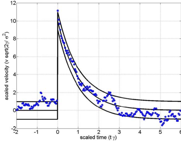
Fig. 6. Points on a sample path of the normalized kicked Ornstein-Uhlenbeck process defined by the Langevin eq. (14). The solid lines represent the mean, and mean \pm standard deviation of the scaled velocity coordinate. At the time t=0 a value of v_0=10 has been added to the scaled velocity. After some time the information of the amplitude gets more and more lost due to the fluctuations.
