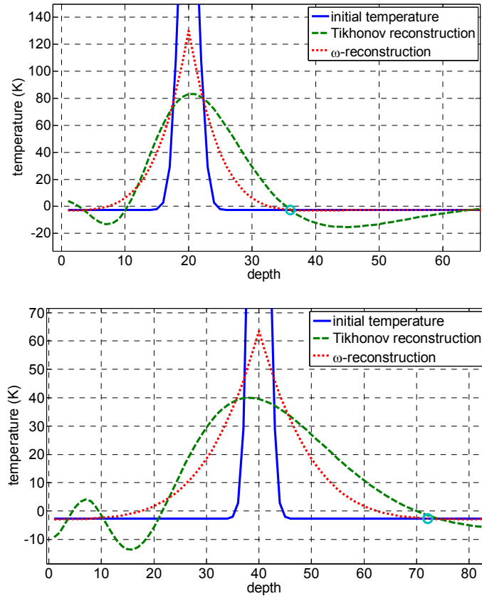
Fig. 24. Comparison of the deviation from equilibrium temperature for Tikhonov reconstruction and “ \omega -space”- reconstruction for a Gaussian initial temperature peak centered at a depth of 20 (top) and at a depth of 40 (bottom). The zero point of the “ \omega -space”- reconstruction, which is the resolution described by eq. (61), is marked by a small circle ‘o’.
