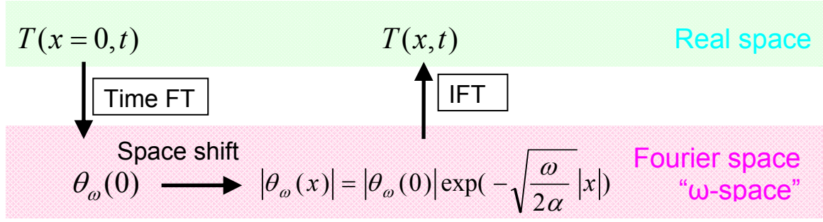
Fig. 20: The temperature T at x=0 is time Fourier transformed (Time FT). The space shifted Fourier series coefficients can be described similar to the mean value of a stochastically damped oscillator process (eq.(28)). The temperature at x is then calculated by an inverse Fourier transform (IFT).
