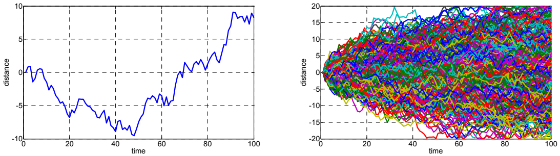
Fig. 2. One realization of the Wiener process with the particle starting at x=0 (left) and 500 realizations using reflecting boundaries at a distance of \pm 20 (right).
