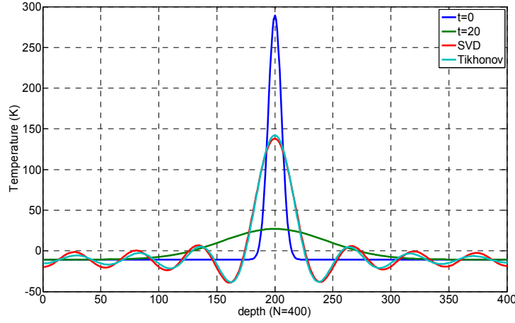
Fig. 17. Reconstruction results for a reduced standard deviation ( 10^{-5} in Fourier space, compared to 1 in Fig. 16).
