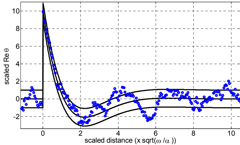
Fig. 19. Points show a realization of the stochastically damped oscillator; the solid lines represent the mean and the standard deviation (see also Fig. 9). The mean value is described by eq. (56). \text{Re } \theta is scaled that its standard deviation is one and the scaled distance is x\sqrt{\omega/\alpha} .
