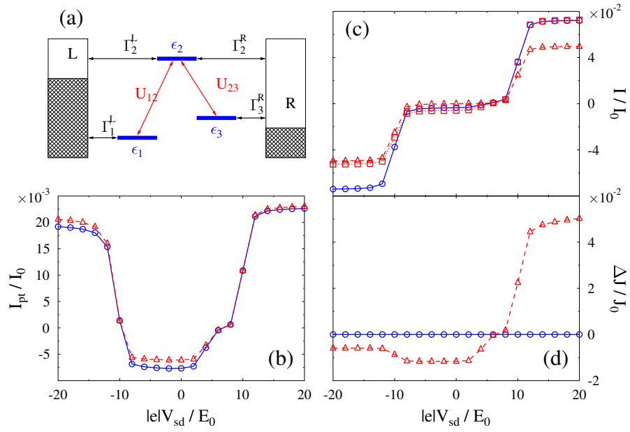
Figure 10: Physical conservation laws in junction spectroscopy. For a three-level model (a) calculations of photon (b) electron (c) and energy (d) fluxes within diagrammatic (solid blue line) and bare (dashed and dotted red lines) perturbation theories show violation of conservation laws by the latter. Reprinted from [Y. Gao and M. Galperin, J. Chem. Phys. 2016, 144 , 174113], with the permission of AIP Publishing.
