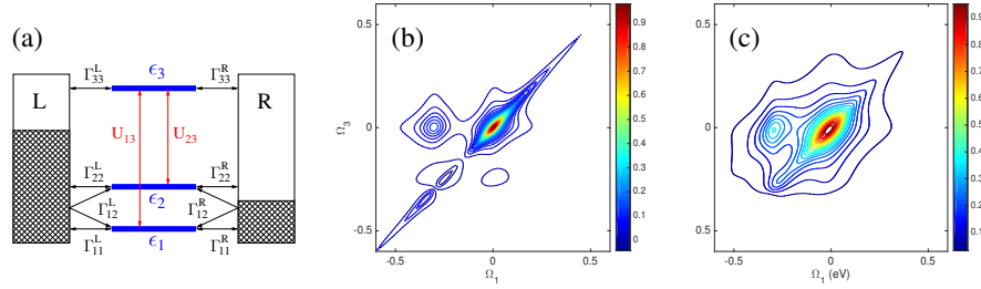
Figure 4: An example of 2D optical signal in a nanojunction. Shown are (a) junction model, (b) NEGF (exact for the model) and (c) PP-NEGF results. Lindblad/Redfield Liouville space formulation yields zero signal. Reprinted from [Y. Gao and M. Galperin, J. Chem. Phys. , 2016, 144 , 244106], with the permission of AIP Publishing.
